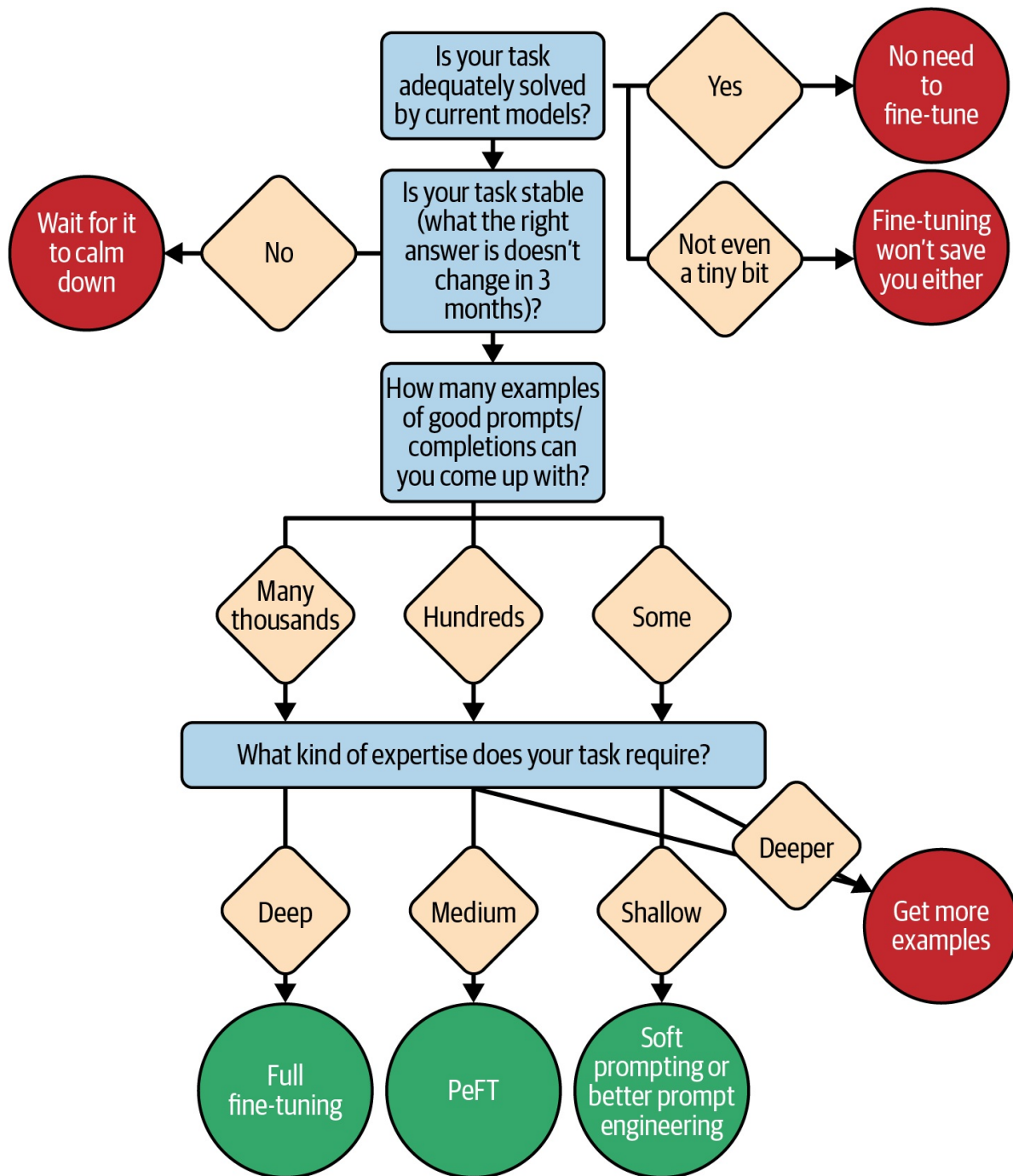
Figure 7-8. Should you fine-tune?
