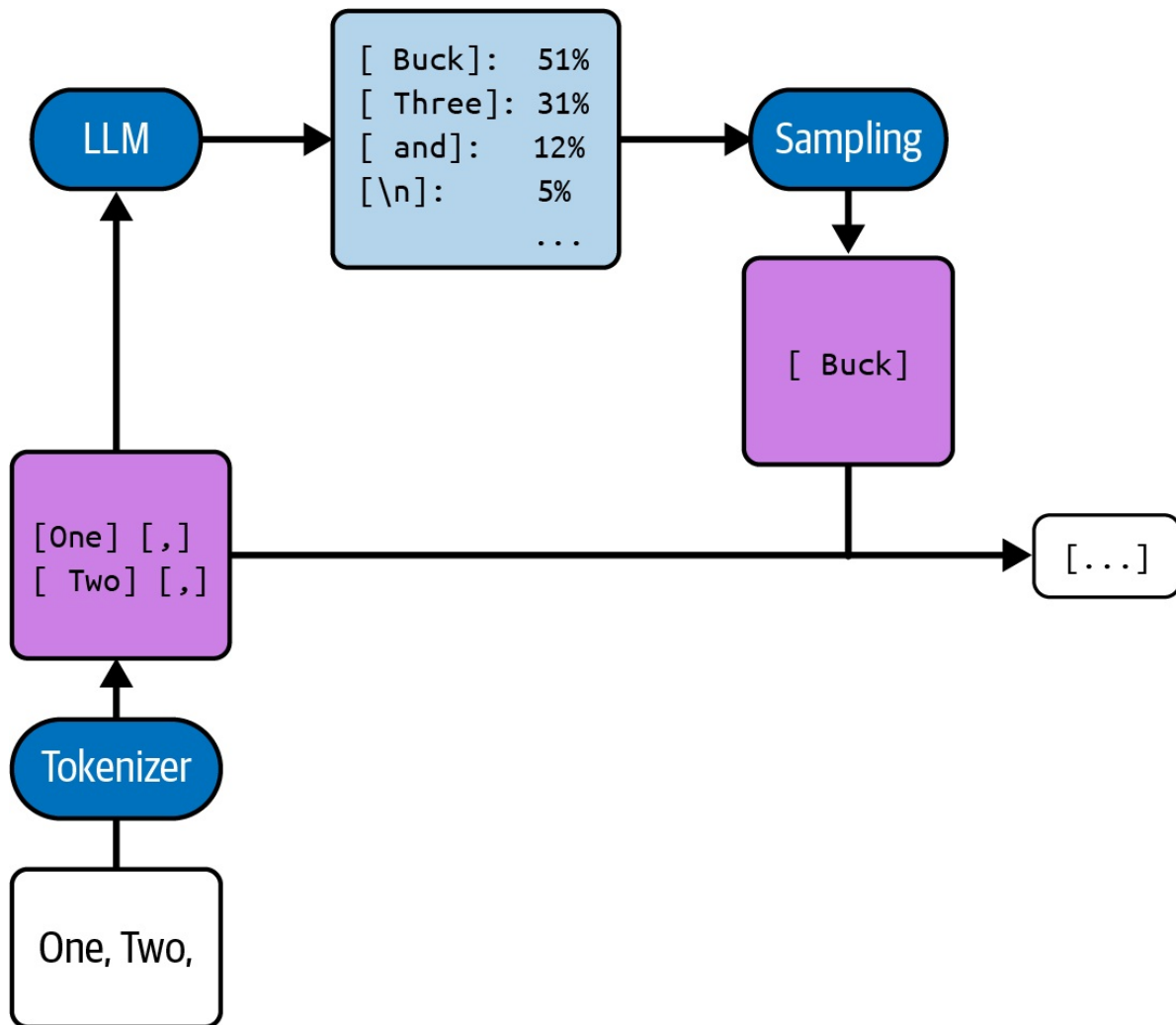
Figure 2-11. The sampling process in action
