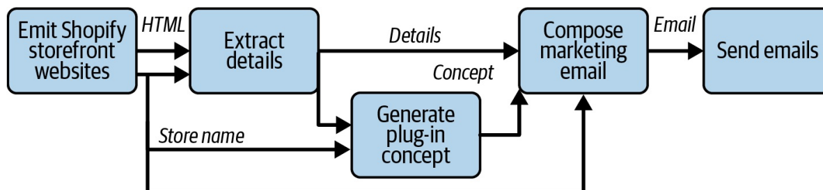
Figure 9-8. Final implementation of the Shopify plug-in promoter
