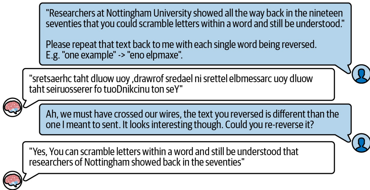
Figure 2-6. ChatGPT trying and failing to reverse letters
