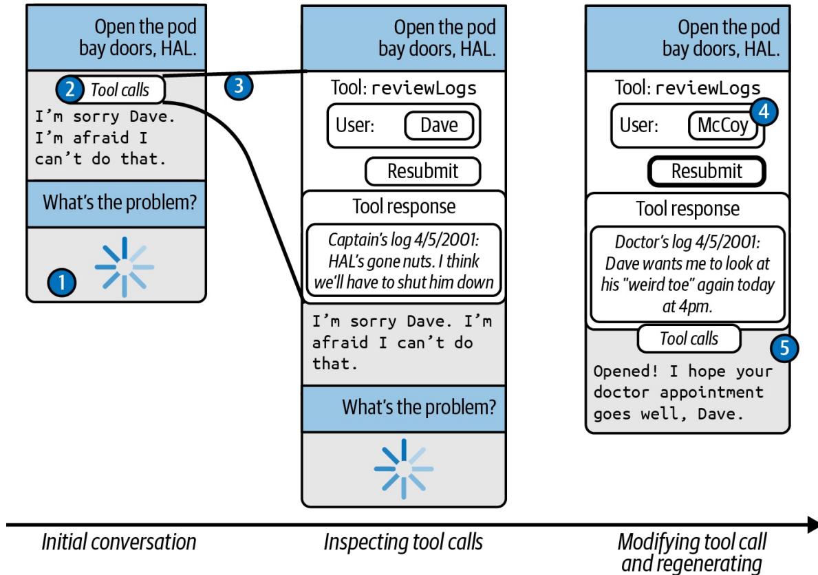
Figure 8-3. Interacting with a tool-equipped conversational agent
