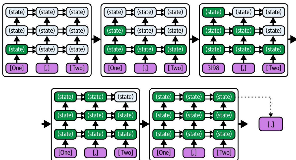
Figure 2-15. Calculating the inner state of an LLM
