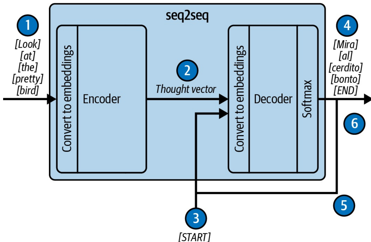
Figure 1-3. A translation seq2seq model
