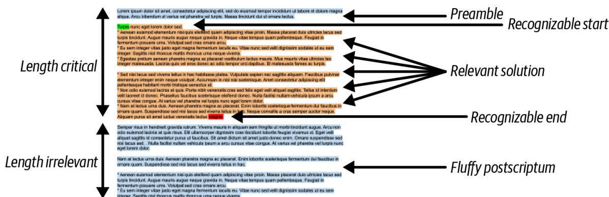
Figure 7-1. An LLM completion
